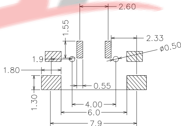
RECOMMENDED P.C.B LAYOUT (TOP VIEW) EFFECTIVE TOLERANCE: ±0.05
