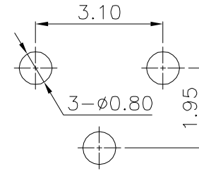
PCP Layout (Pattern Side)
