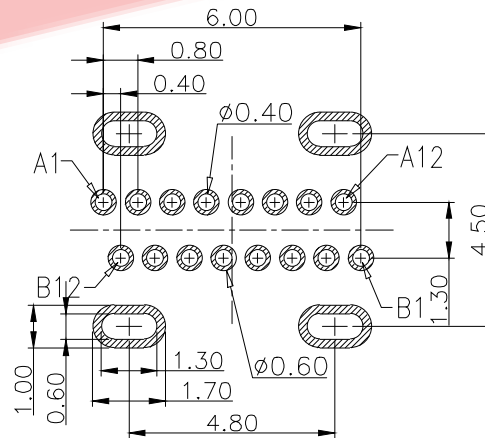
RECOMMEND P.C.B LAYOUT TOLERANCE UNSPECIFIED ±0.05mm
